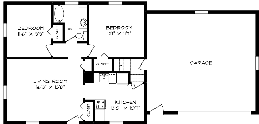
MAIN FLOOR 850 SQUARE FEET
